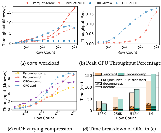
Figure 16: GPU Decoding
